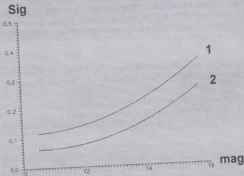
Figure 1: The instrumental accuracy of coordinate determination with CCD as a function of magnitude (in arcsecor
