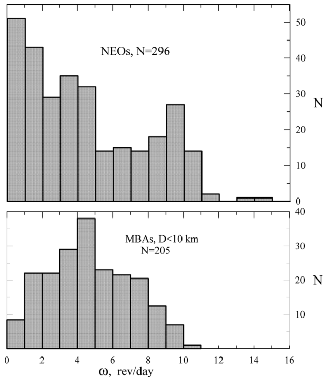
Figure 1. Distribution of the rotation rates of NEOs and small ( D \leq 10 km) MBAs.
